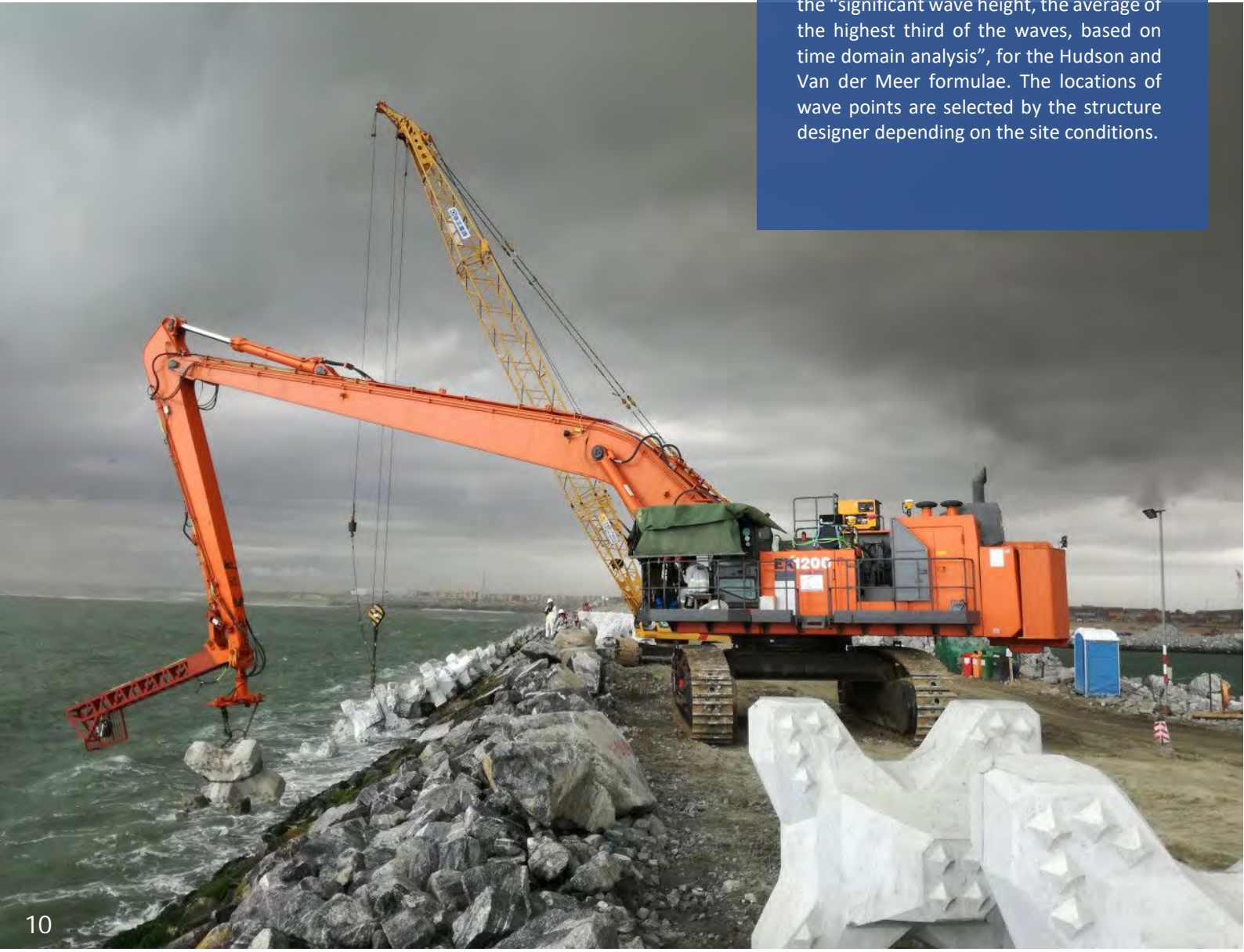
Figure 5: Hydraulic shovel and lattice boom crawler crane during ACCROPODE™ II unit placing
