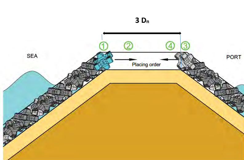
Figure 28: Example of a completely covered crest
