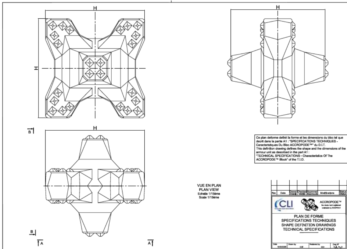
Figure 2: ACCROPODE™ II unit drawings
